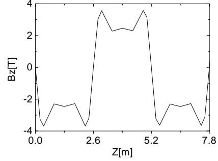
Figure 2: Magnetic field B_z [T] in the cooling channel.
