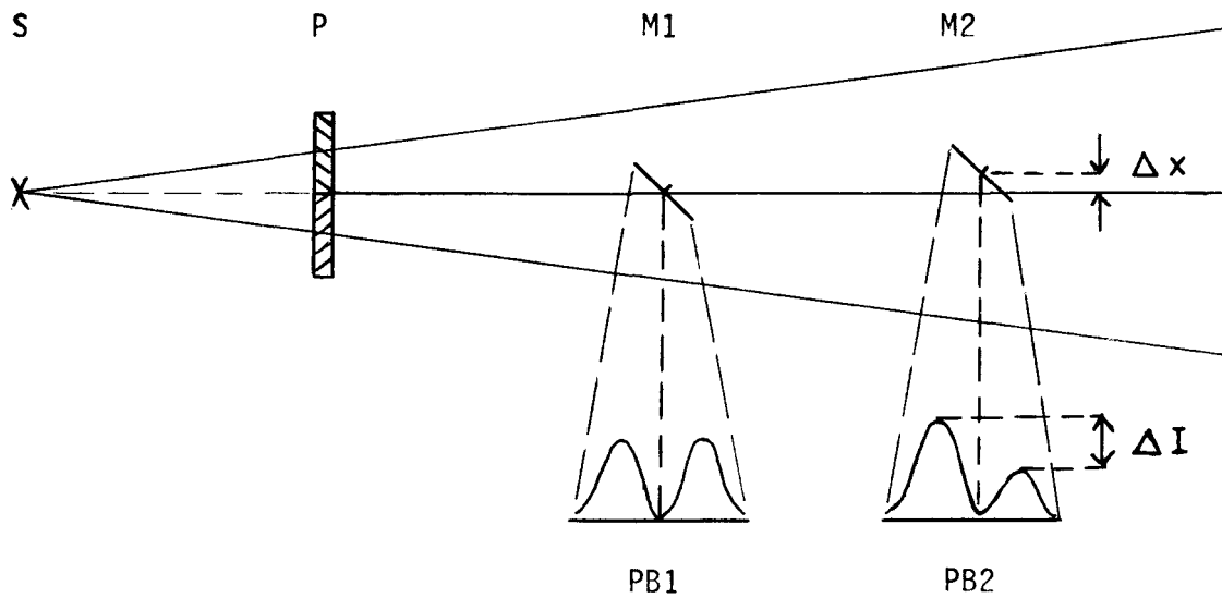
Fig. 5: Asymmetry method with variable detection plane and simultaneous alignment control (M1, M2 = mirrors).
