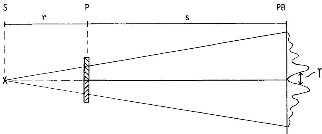
Fig. 1: Demonstration of the minimum principle. (S=laser source, P=phase plate, PB=plane of observation).
