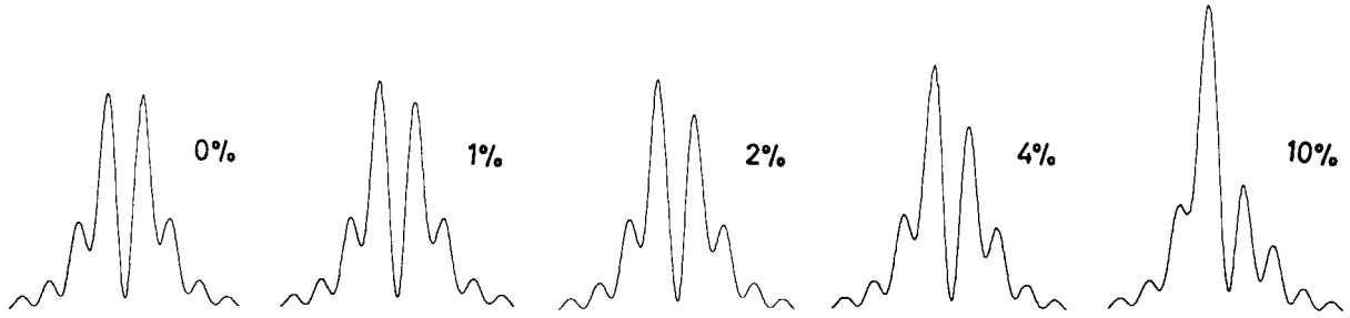
Fig. 3: Experimental intensity distribution, obtained at PB with the asymmetry method in one dimension. The slit to be aligned in the plane PA was displaced 0%, 1%, 2%, 4% and 10% of its width.
