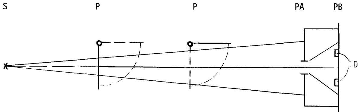
Fig. 4: Schematic diagram for an alignment system based on the asymmetry method with fixed detection unit (D=detectors).
