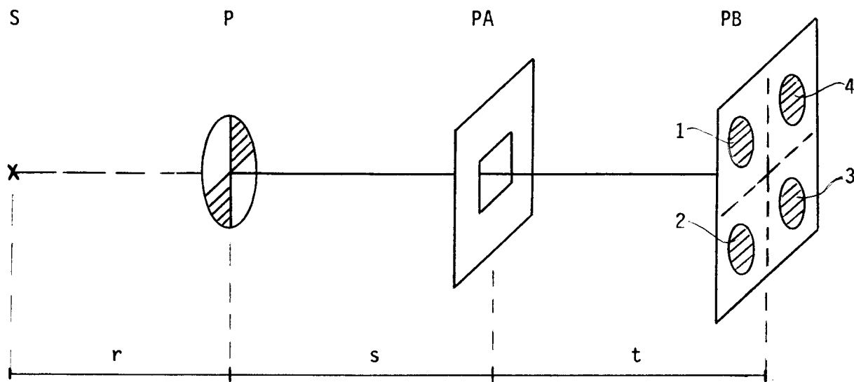
Fig. 2: Principle of the asymmetry method in two dimensions.
