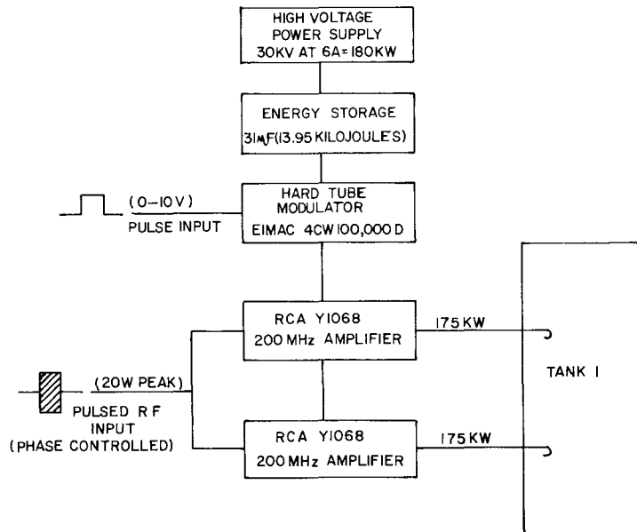
Figure 2 — RF Power System for Cavity No. 1
