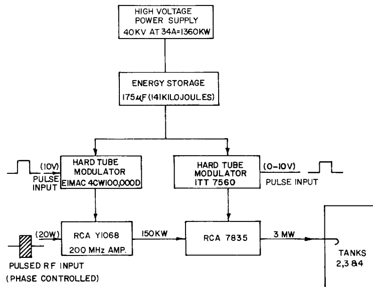
Figure 3 — RF Power System for Cavities 2, 3, and 4
