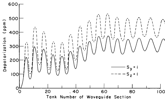
Fig. 2. Same as Fig. 1. with different initial conditions on the spin vector.
