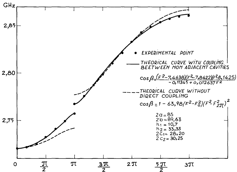
Figure 10- Calculated and measured dispersion curve for the triperiodic structure of type I.
