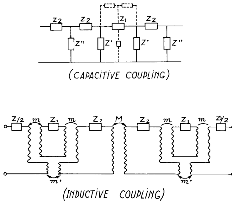
Figure 2 - Equivalent circuits used to represent the triperiodic structure.
