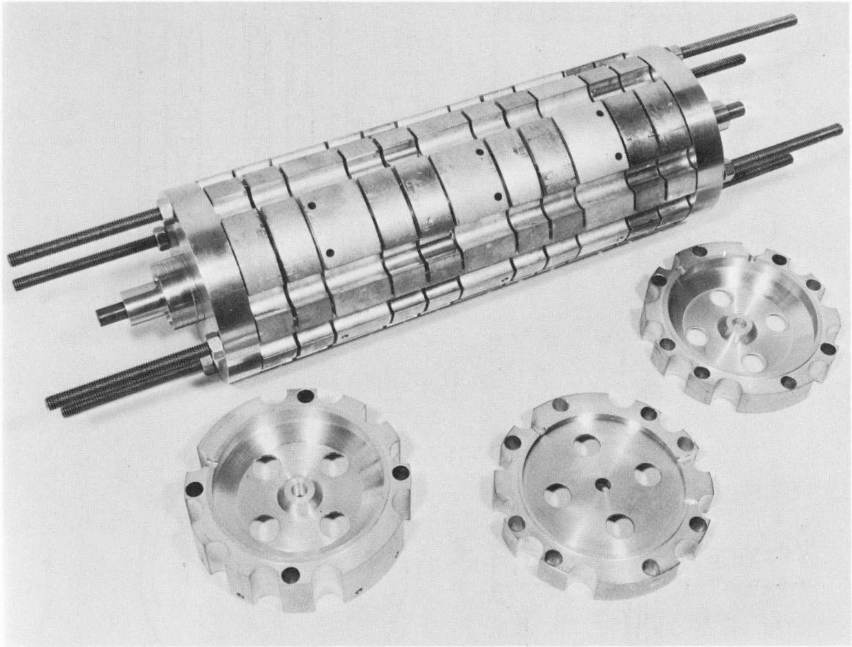
Figure 5 --Type II structure.
