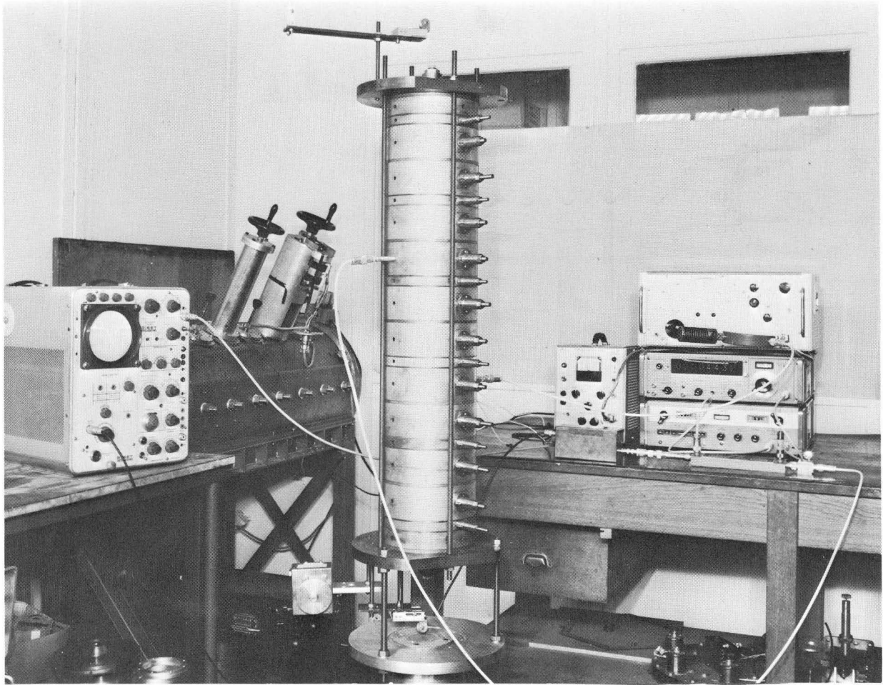
Figure 7 - Assembled cavity.
