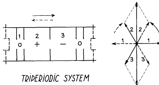
Figure 1 - Schematic representation of bi and triperiodic structures. The forward and backward waves are represented by solid and dashed arrows respectively.
