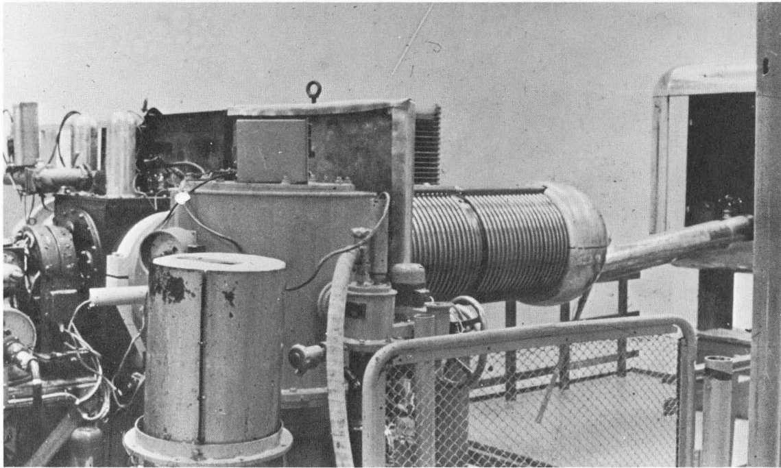
Fig.3 700 keV Accelerating Tube and Vacuum Chamber
