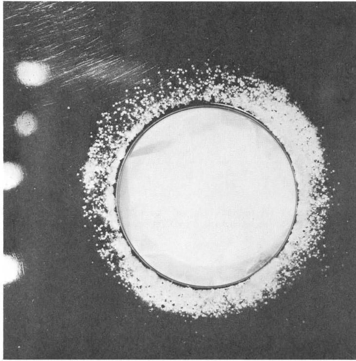
Fig. 6 Craters around the cathode beam hole.
