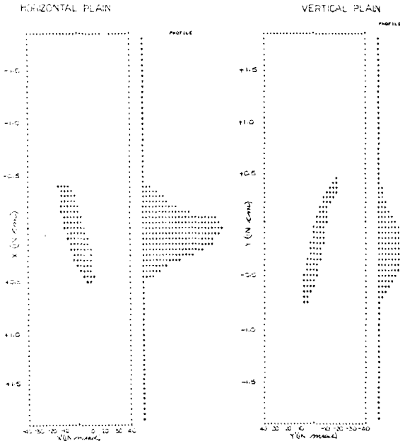
Fig. 3. Measured 10 MeV emittance.
