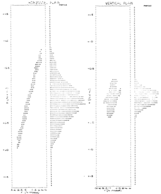
Fig. 2. Measured 0.750 MeV emittance
