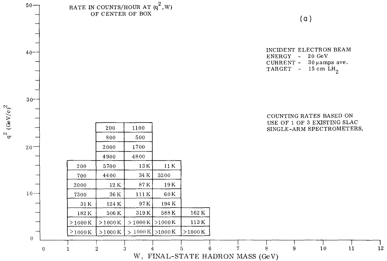
Figure 5. Expected counting rates for inelastic scattering using single arm spectrometers with the present SLAC accelerator (a) and RLA (b).
