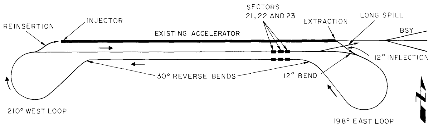
Figure 1. Schematic layout of the recirculating linear accelerator.
