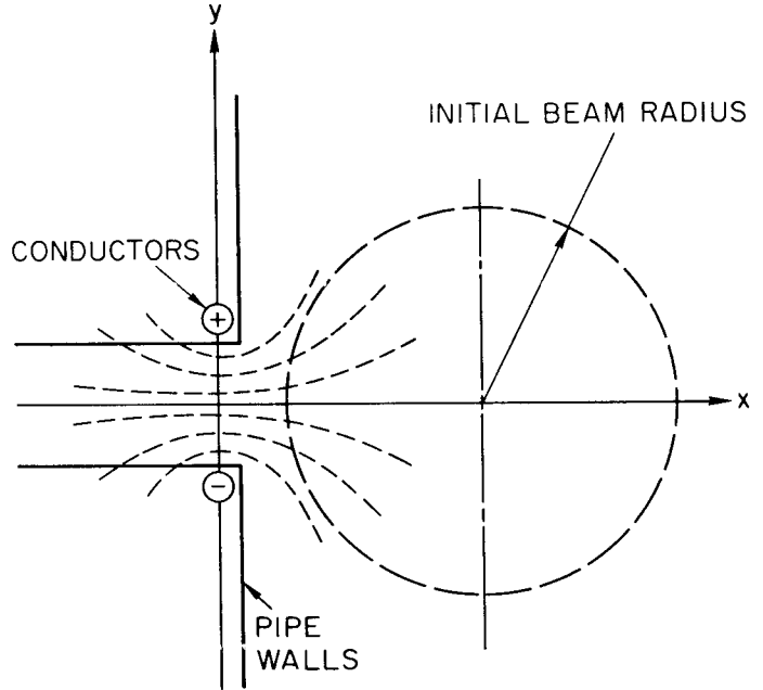
Figure 4. Bifilar loop for magnetic perturbation suitable for a long spill extraction device.
