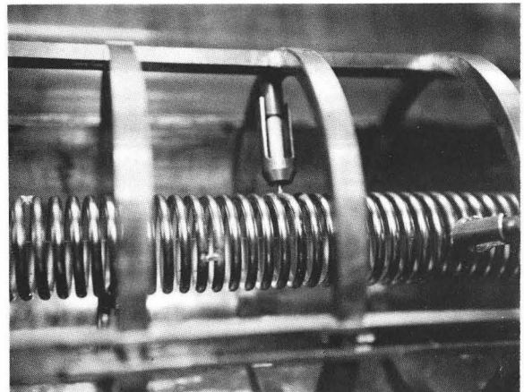
Fig. 2. Part of a compensated helix structure.
