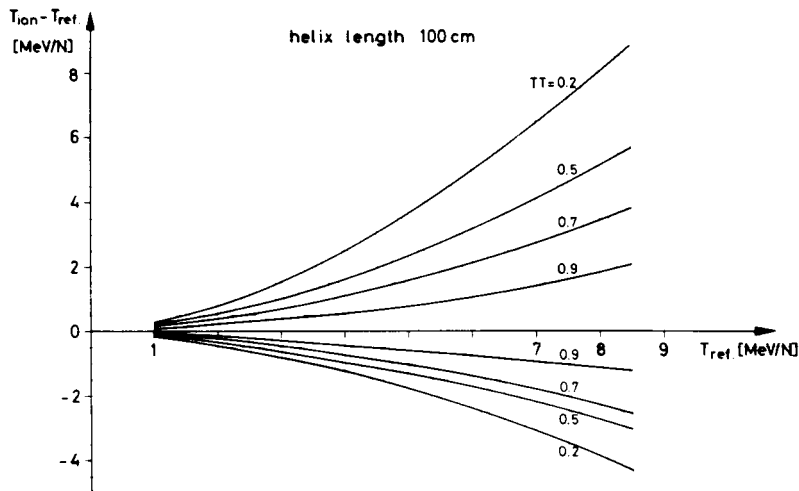
Fig. 8. Dependence of transit time factor on the energy ( v_{\text{phase}} = v_{\text{particle}} ).
