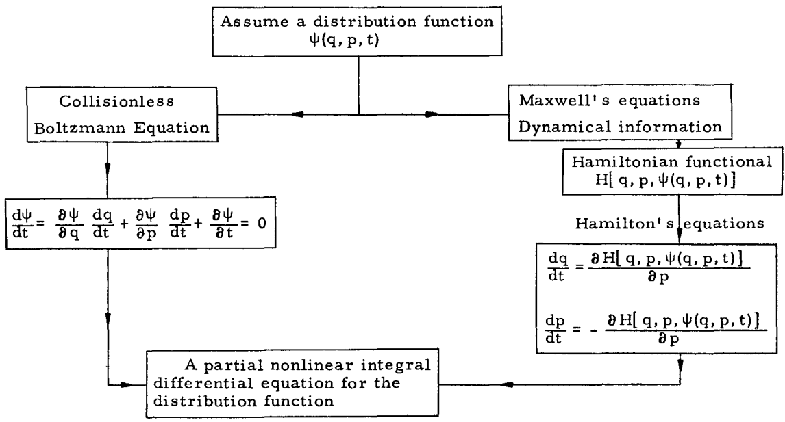
Figure 2 Block diagram of the collisionless Boltzmann equation approach to self-field phenomena
