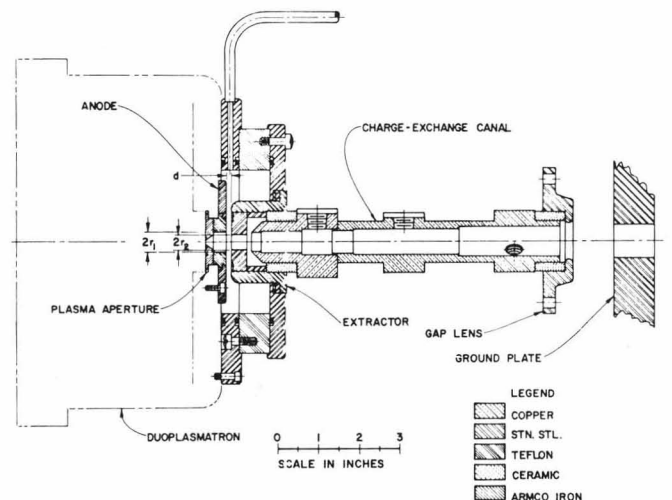
Fig. 4. Single aperture extraction H^- ion source employing flat plate electrodes.
