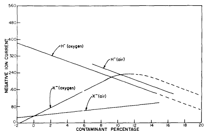
Fig. 2. H^- and heavy negative ion yield vs percentage air or oxygen in the duoplasmatron arc chamber at 15-kV extraction voltage. Data points have been eliminated for clarity, and the heavy ion yield has been extrapolated to zero, indicating about 2% contamination of the arc under normal operating conditions.
