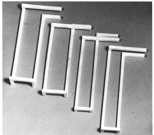
Fig. 13 Insulated coil turns, TR-BM-02
