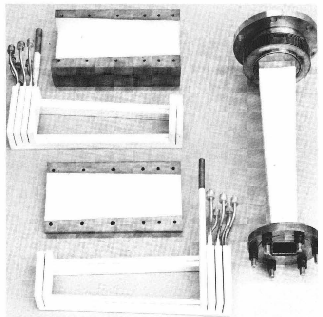
Fig. 7 Magnet components, TR-BM-01, 04
