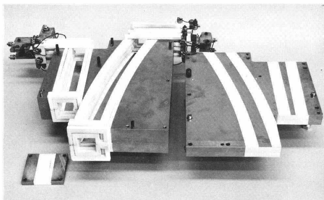
Fig. 16 Magnet partial assembly, TR-BM-02. 06
