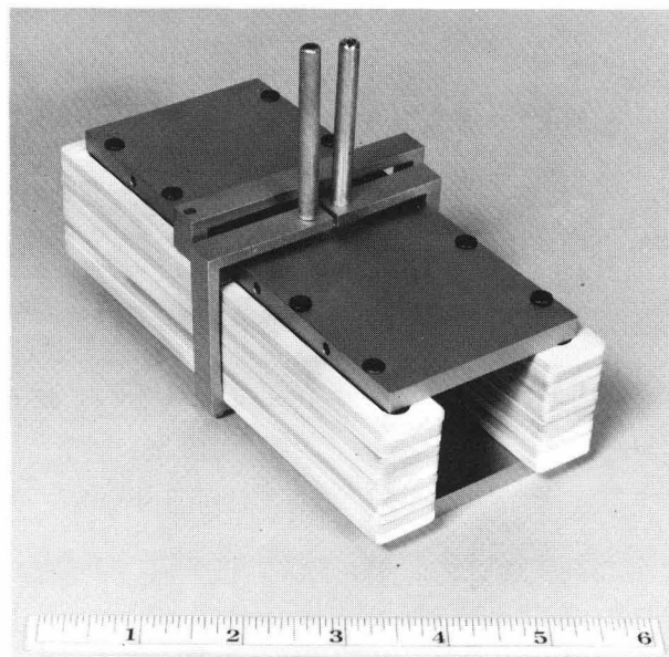
Fig. 2 Drift tube steering magnet assembly
