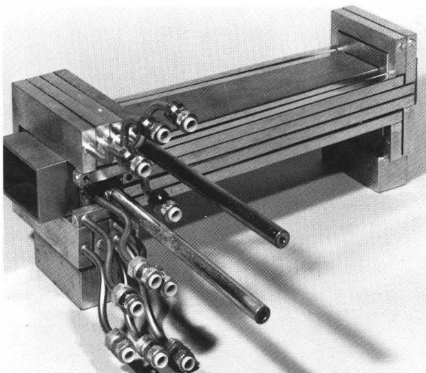
Fig. 6 Brazed coil assembly, TR-BM-01, 04
