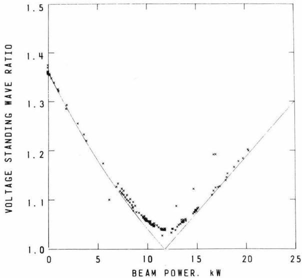
Fig. 5 Variation of voltage standing wave ratio in the transmission line to the structure with incremental beam power. The points are measured values and the smooth curve is the theoretical best fit for critical coupling at 11.7 kW.
