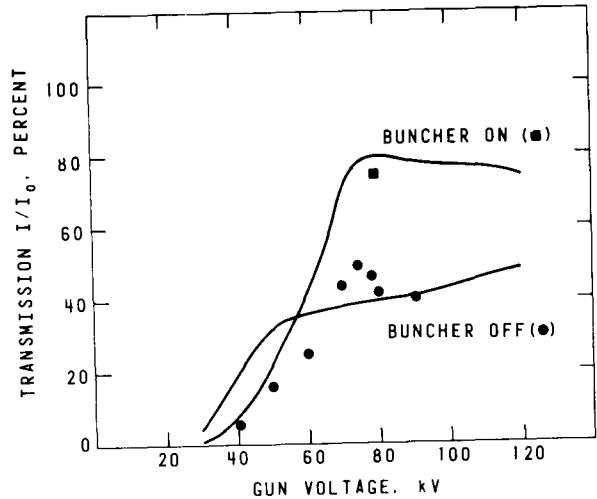
Fig. 1 Beam transmission vs. gun voltage with and without the buncher operating. I is the current in a Faraday cup at the output of the accelerator and I_0 is the dc current from the gun. The curves were calculated, the solid circles measured with buncher off and the single square point measured with buncher on and with the normal gun voltage.
