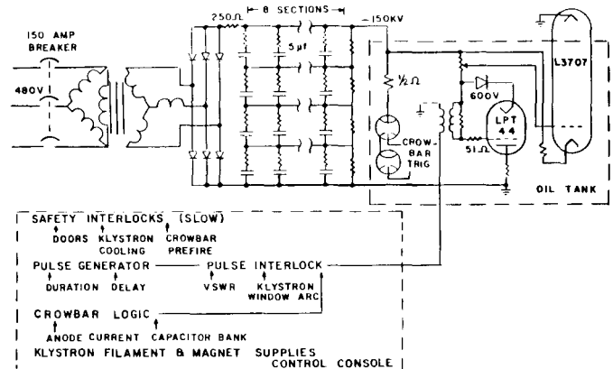
Fig. 2. Electrical schematic of rf modulator.
