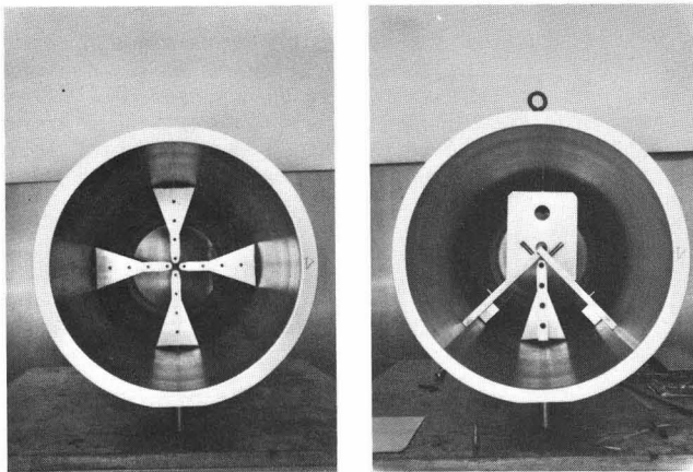
Fig. 4. Full-scale model a) with four vanes mounted b) with single isolated vane.
