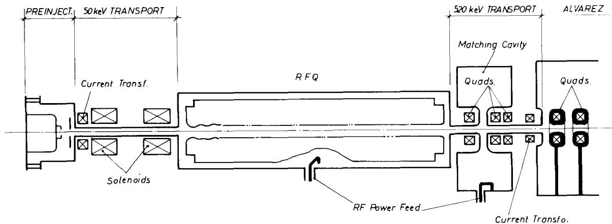
Fig. 1. Schematic layout.
