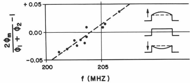
Fig. 5. Nonlinear term versus frequency.
