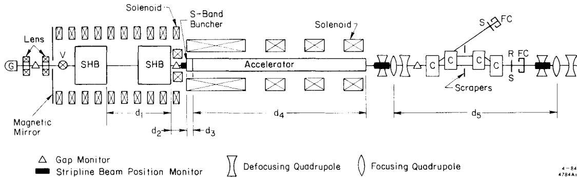
Fig. 1. Schematic drawing of the SLC electron source. Abbreviations which have been used are as follows: C, compressor magnet; FC, Faraday cup; G, gun; L, lens; R, Čerenkov radiator; S, screen for profile monitor; V, valve. The distances d_1 through d_5 are 108, 30, 10.3, 300 and 400 cm respectively. The quadrupole focusing refers to the horizontal plane.
