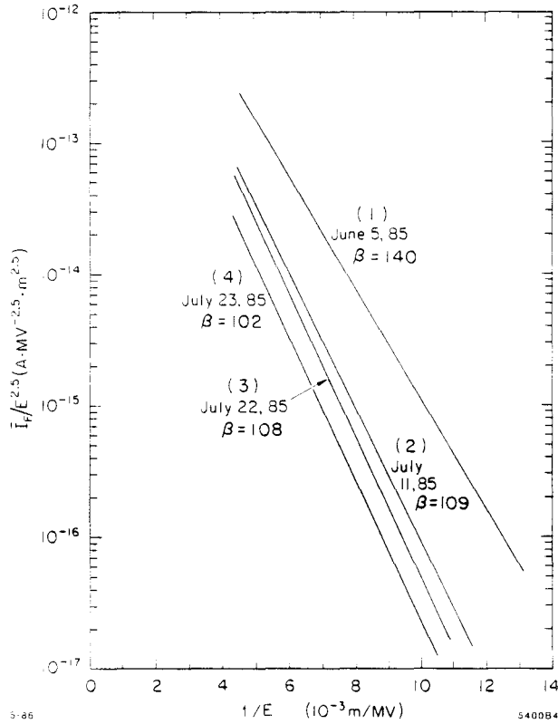
Fig. 7. Modified Fowler-Nordheim plots.
