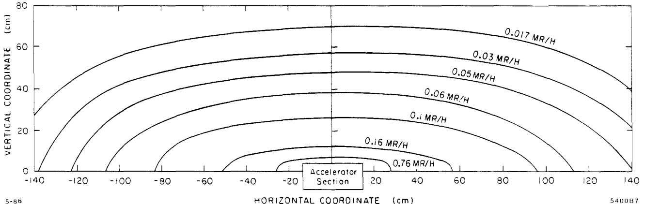
Fig. 6. X-ray dosage distribution around accelerator section (300 MV/m surface field, 2.5 μsec, 120 pps).
