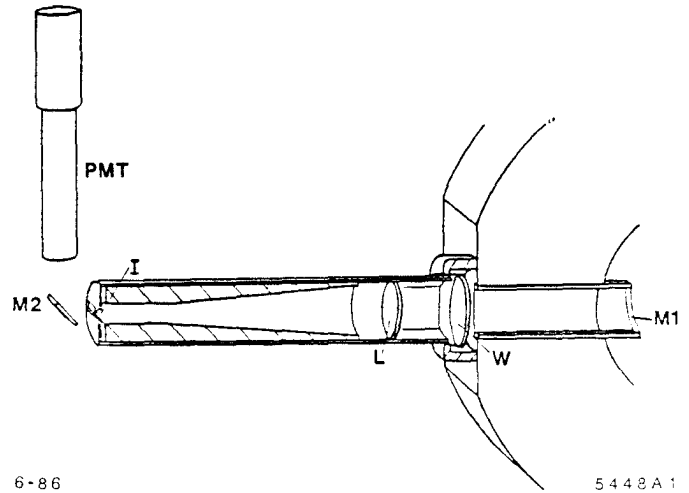
Fig. 1. Beamstrahlung periscope: M1 is the primary mirror, W the vacuum window, L the lens, I the iris, and M2 a 45^\circ mirror. The surrounding radiation shielding is not shown.
