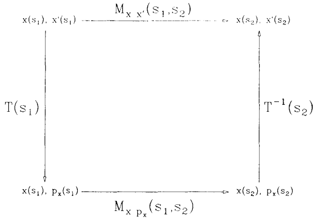
Figure 1 Relation Between Canonical and Non-Canonical Representations
