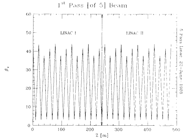
Figure 3 Transport of Non-Canonical Beta Function
