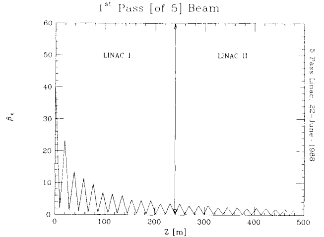
Figure 2 Transport of Canonical Beta Function
