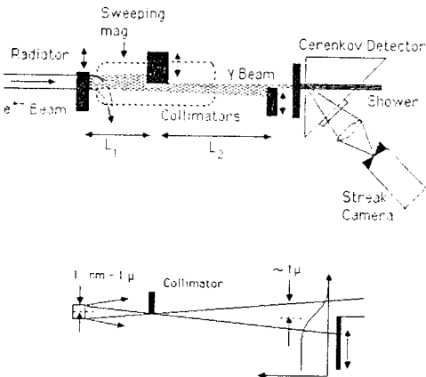
Fig. 1 Plan of Bremsstrahlung Monitor
