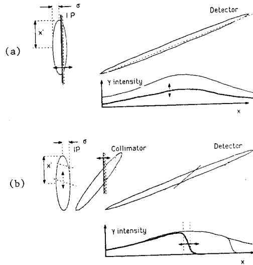
Fig. 2 Photon Phase Space
