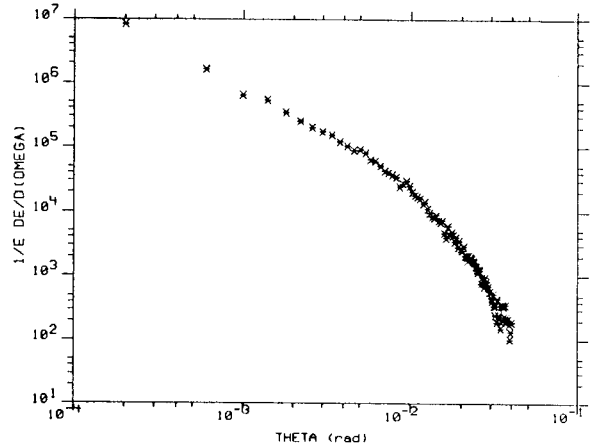
Fig. 3 Angular distribution for slit scattering, 1/E \text{ dE/d}\Omega , for 1 TeV a beam.
