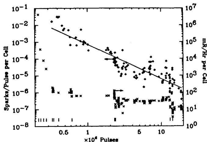
Fig. 3. Sparking rate ( \diamond ) and x-ray production ( \times ) as a function of conditioning time as measured by the number of pulses in Prototype 2. Each have been corrected for pulse length and normalized to 37.1 MV/m. The ticks along the bottom indicate when a new electric field was achieved for the first time. The line is fit to the sparking rate for the interval between 500,000 and 19 million pulses and has a slope of -2.
