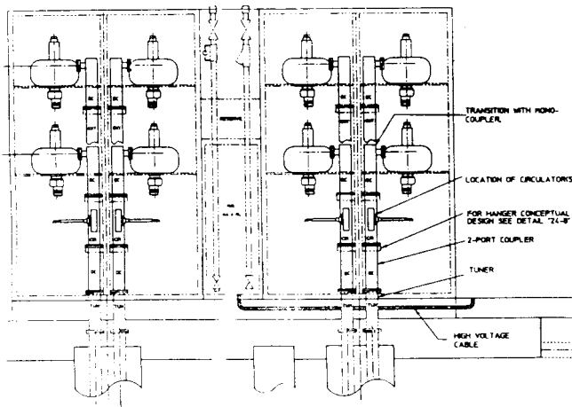
Figure 3. Location of klystrons and waveguide components.
