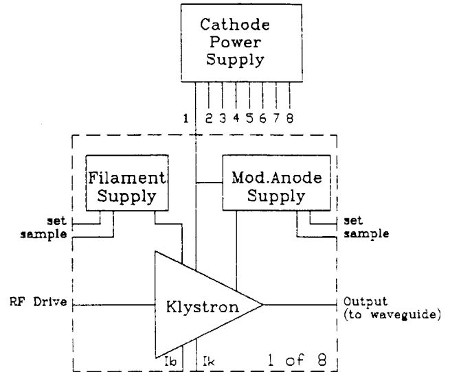
Figure 4. Simplified block diagram of power sections of HPA.
