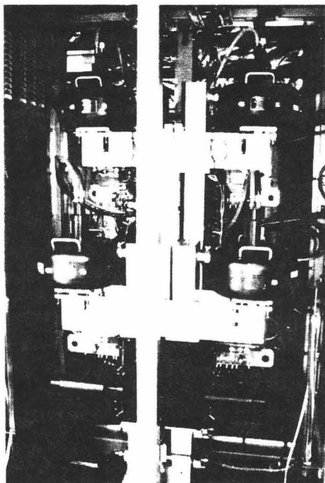
Figure 2. Four of eight klystrons installed along with associated waveguide.
