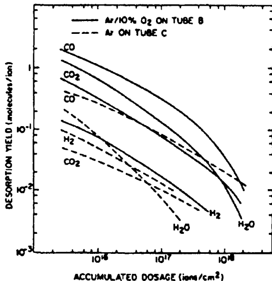
Fig. 10. Glow discharge cleaning of stainless steel tubes at Brookhaven ring.
