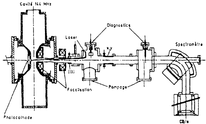
Fig. 5. Photoinjector designed at LEL-HF Bruyeres-le-Chatel
