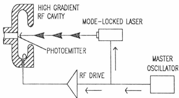
Fig. 1. Schematic of a photoinjector.
