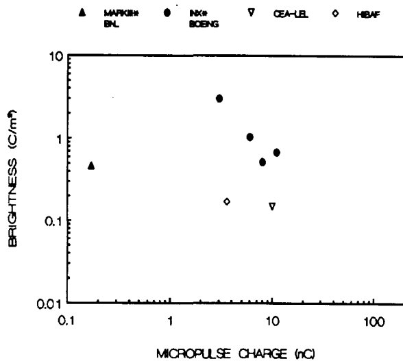
Fig. 7. Photoinjectors - experiment results.
