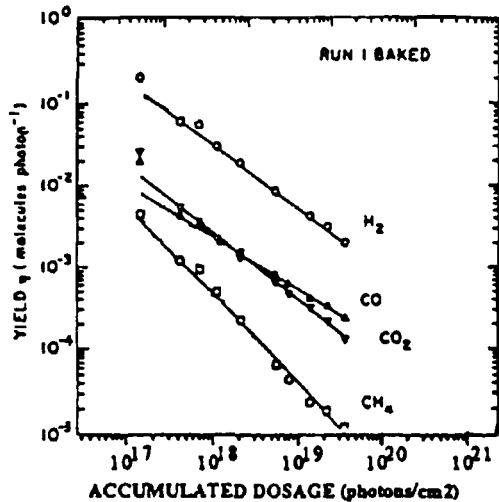
Fig. 9. Photodesorption yield during beam conditioning for Al at NSLS VUV storage ring.
