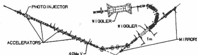
Fig. 3. Upgrade of Los Alamos FEL accelerator with photoinjector: HIBAF.
