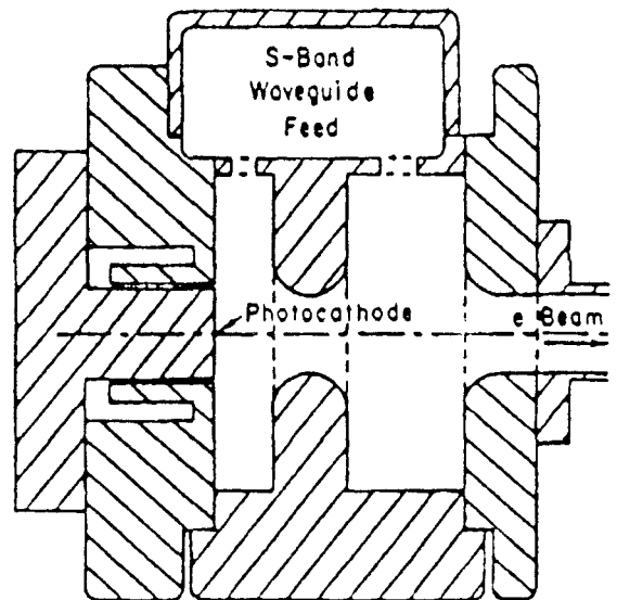
Fig. 6. Schematic of BNL photoinjector.
