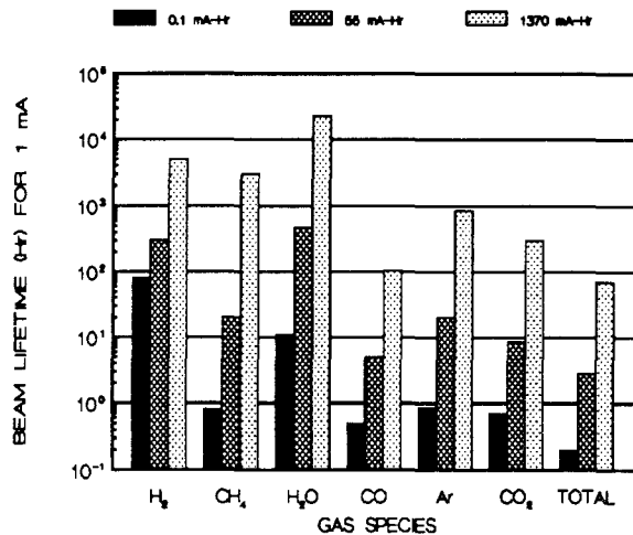
Fig. 11. Data from the electron positron accumulator ring at CERN.
