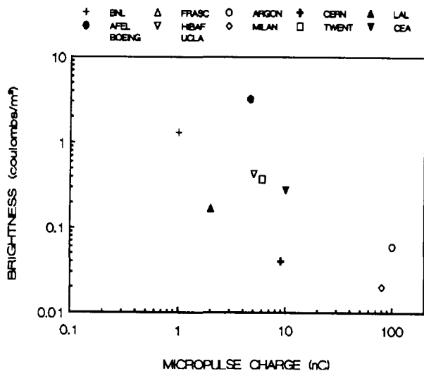
Fig. 8. Photoinjectors - planned experiments.
