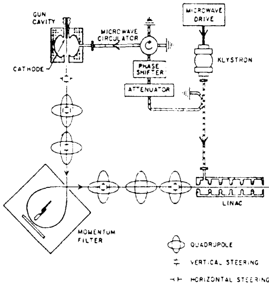
Fig. 4. Schematic of Mark III accelerator.
