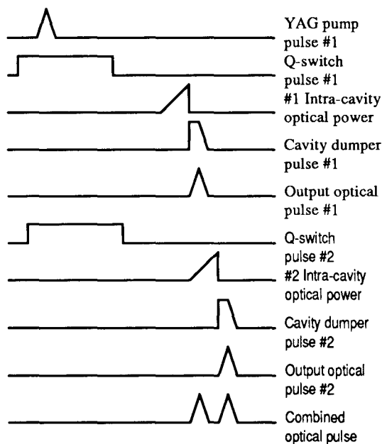
Fig. 2 System pulse timing.
