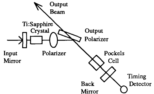
Fig. 3 Ti:Sapphire cavity design
