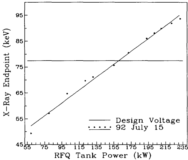
Fig. 4 X-ray measurements.
