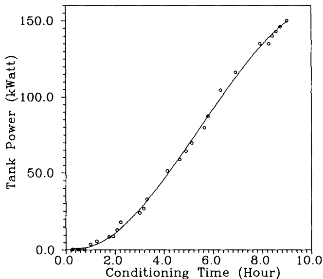
Fig. 2 High-power conditioning versus time.
