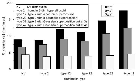
Fig. 8. Rms-emittance for different input particle distributions.
