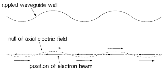
Fig. 2. Axial electric field orientations for a synchronous particle when the particle reaches the centers of the ripples in r-z geometry.
