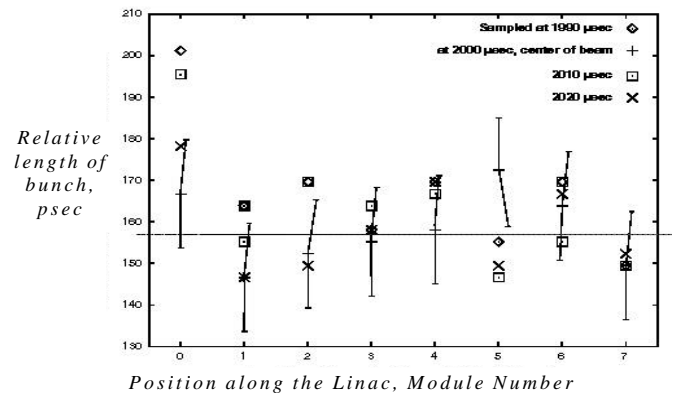
Figure 1, Measurement results from Wall-current Monitors
