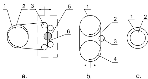
Fig.8. Targets with "running" and "boiling" wires.
