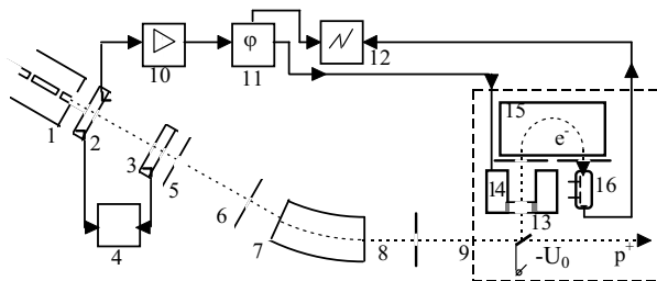
Fig.1. Emittance measurement system
