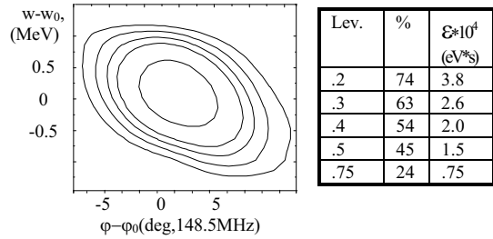
Fig.2. Emittance of the I-100 linac beam.
