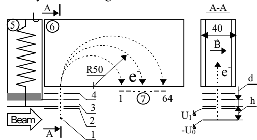
Fig.3. Layout of BPD detector.
