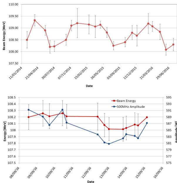
Figure 3: Thermal effects are observed on the linac beam energy. Above: long term temperature variations. Below: day-to-day variations, correlated with the 500MHz amplitude that feeds PB1. Both thermal effects do not affect the injection to booster.
