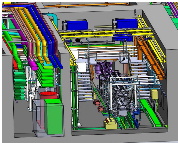
Figure 4: 3D views of processes + connections + buildings.
