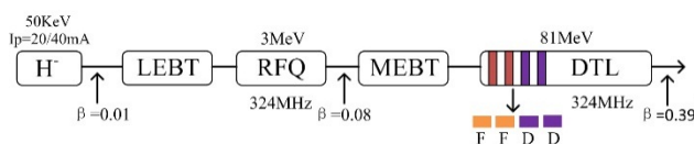
Figure 1: CSNS Linac injectors.
