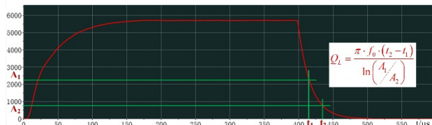
Figure 4: Selecting two A(t) values for calculating Q L .
