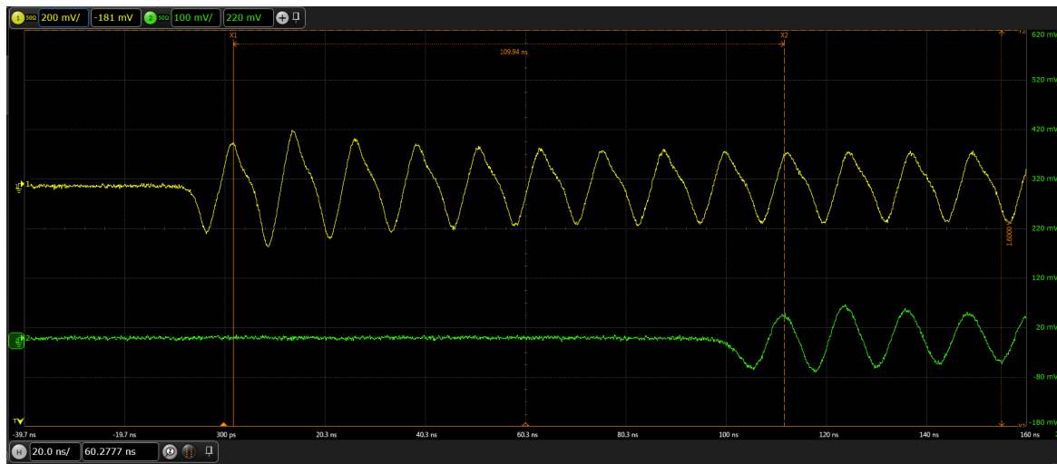
Figure 5: Measured signals of N 2+ beam current form two BPMs.
