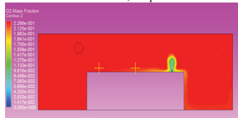
Figure 8: Simulation results of oxygen mass fraction.
