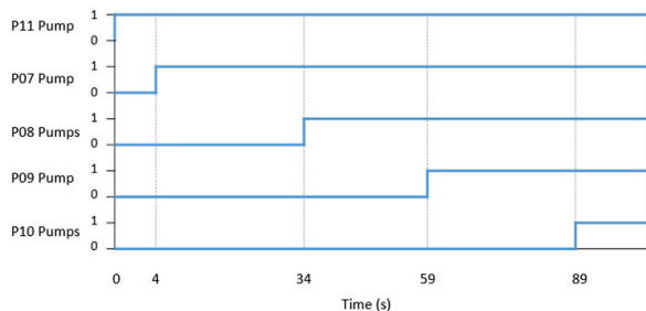
Figure 2: Selected instants of time for each pumping station start-up based on current practice by ALBA operators.
