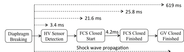
Figure 3: Flow chart for a series of event accompanying the FCS action, along with typical actual values in the case of basic configuration (35PP only) as an example.
