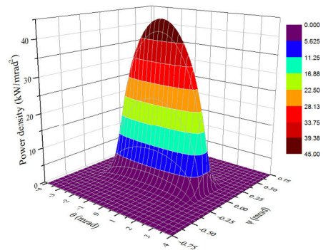
Figure 1: Power distribution of SCW.
