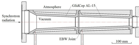
Figure 7: FM (EBW).
