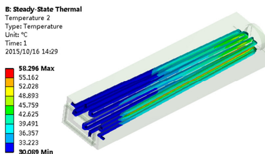
Figure 5: Temperature distribution of the cooling channel walls for FM2.
