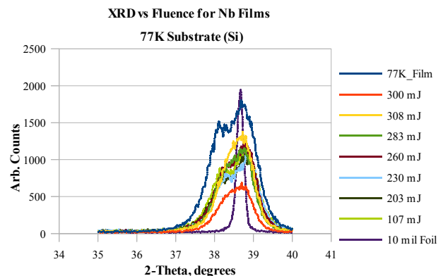
Figure 2: Bragg angle XRD data for raw and processed films, for various fluences. Double peaks resolve, and narrowing is seen for ~300 mJ/cm 2 films. Scherrer grain size doubled from 4 nm to 9 nm during processing. Bulk Nb foil is included as a comparison, as well as a fiducial.
