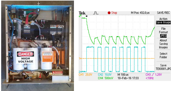
Figure 1: MPPMS modulator (left), and oscilloscope trace of a single MPPMS macropulse, for voltage (green, Volts) and gate drive (blue).
