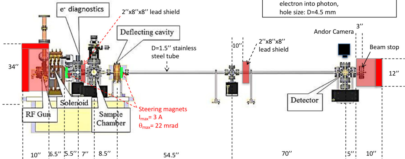
Figure 2: The layout of the initial operational configuration of the UED apparatus in Building 912 at Brookhaven National Laboratory.
