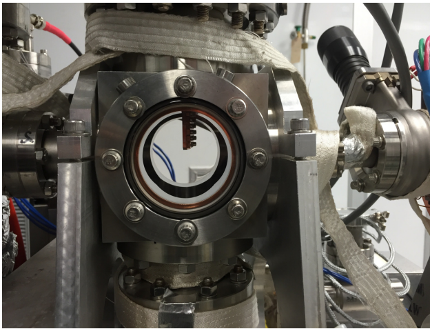
Figure 4: The UED sample holder. The holder utilizes a “cartridge system” to hold multiple samples for efficient user operations.
