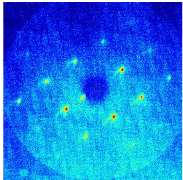
Figure 3: An early diffraction pattern obtained during UED beam line commissioning in June 2016.
