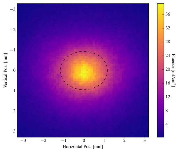
Figure 3: Beam intensity imaged by an intensified CCD camera. The beam is intercepted by an Al 2 O 3 scintillator at the target plane. The dotted line shows the 2\sigma rms radius.
