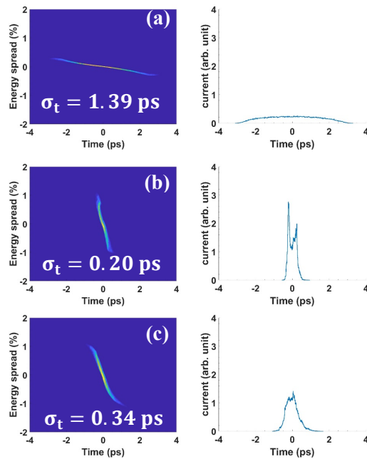
Figure 2: Longitudinal phase spaces and corresponding current profiles without CSR. (a) corresponds to before the DEEX beamline while (b) and (c) corresponds to after DEEX beamline. Octupole correction is not applied to (b) while (c) is the simulation result with octupole correction.
