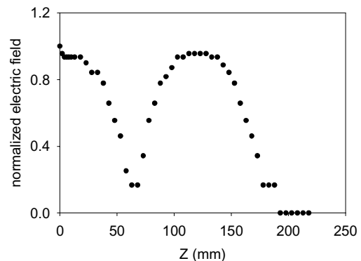
Figure 4: Profile of axial electric field along the axis of the cavity.
