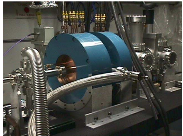
Figure 3: Gun installed in test area.
