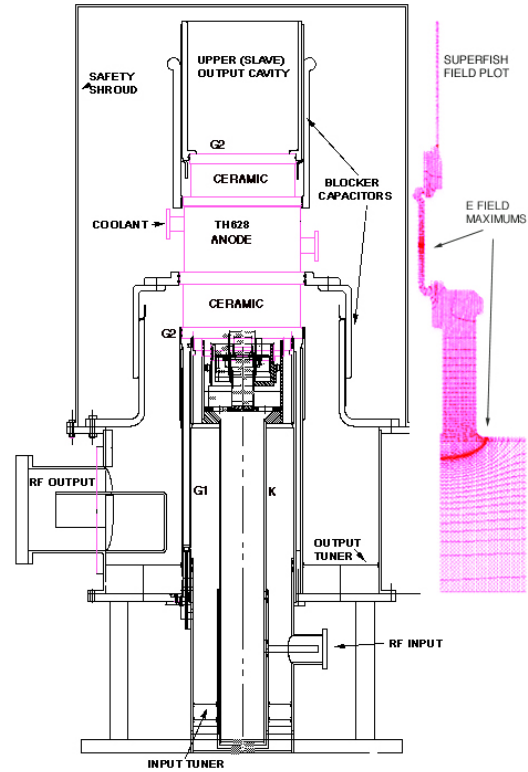
Figure 3: Diagram of Amplifier and Field Plot
