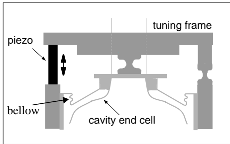
Fig.2: Experimental set-up of PZT integrated with mechanical motor driven frequency tuner.
