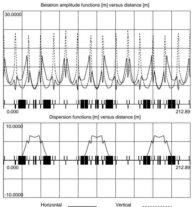
Figure 2 Lattice functions of the RCS
