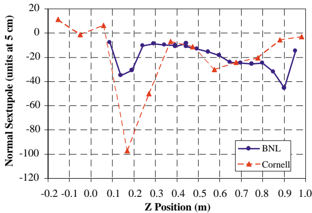
Figure 2: Sextupole distribution measured along the magnet axis.
