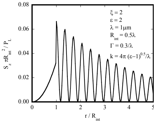
Figure 3: Transverse variation of the energy flux.
