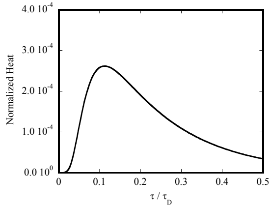
Figure 2: The variation in time of the normalized heat flow at r = R_{\text{ext}} .
