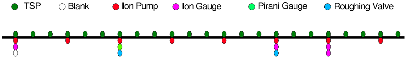
Figure 1: The Recycler Ring Vacuum pump configuration for major portions of the Ring. The remaining portions are being upgraded to have the same configuration. Besides the periodic array of pumps, there are special ion pumps and TSPs installed at critical locations such as Lambertson magnets, stochastic cooling tanks, Schottky detectors etc.
