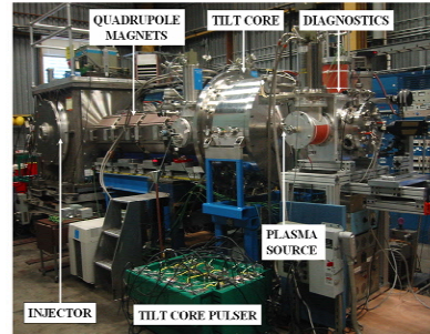
Figure 1: A viewgraph of NDCX-Ia beam line.
